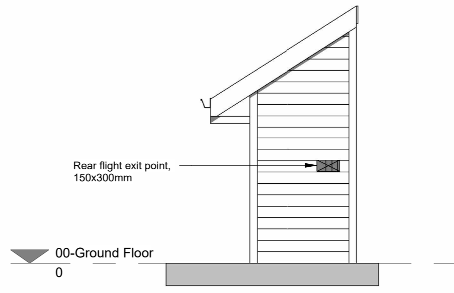
4 Side Elevation - Exit Point 1 : 50
