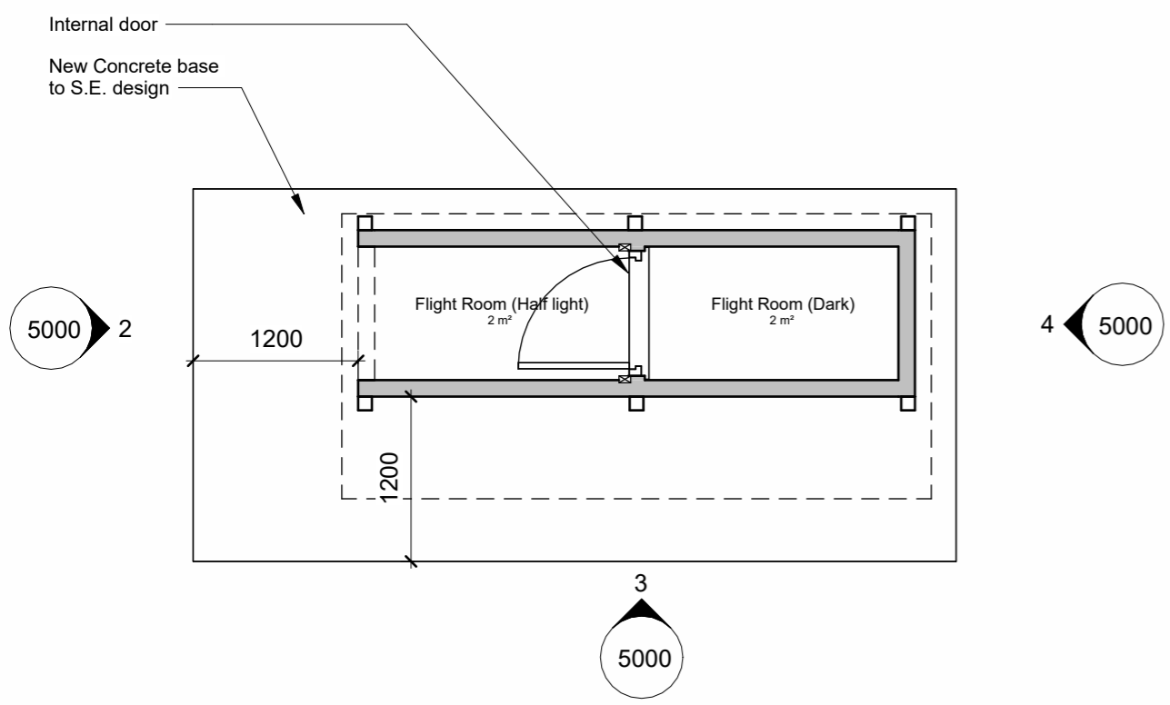
1 Proposed Flight Room Plan 1 : 50
