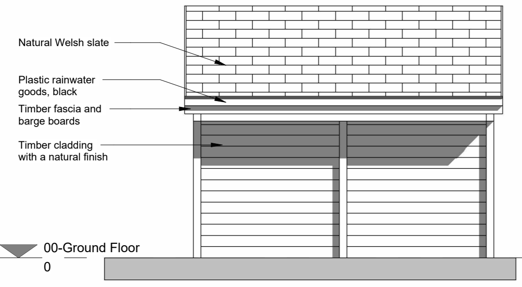
3 Front Elevation 1 : 50
